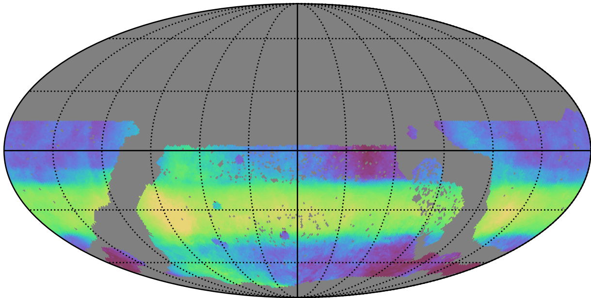
too_elab_r128_d2_griz_v3.4_10yrs WFD all bands: Median HA
