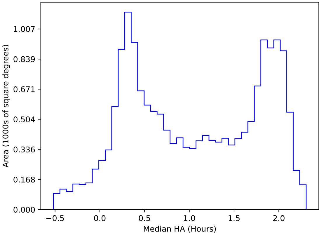
too_elab_r128_d2_griz_v3.4_10yrs WFD all bands: Median HA
