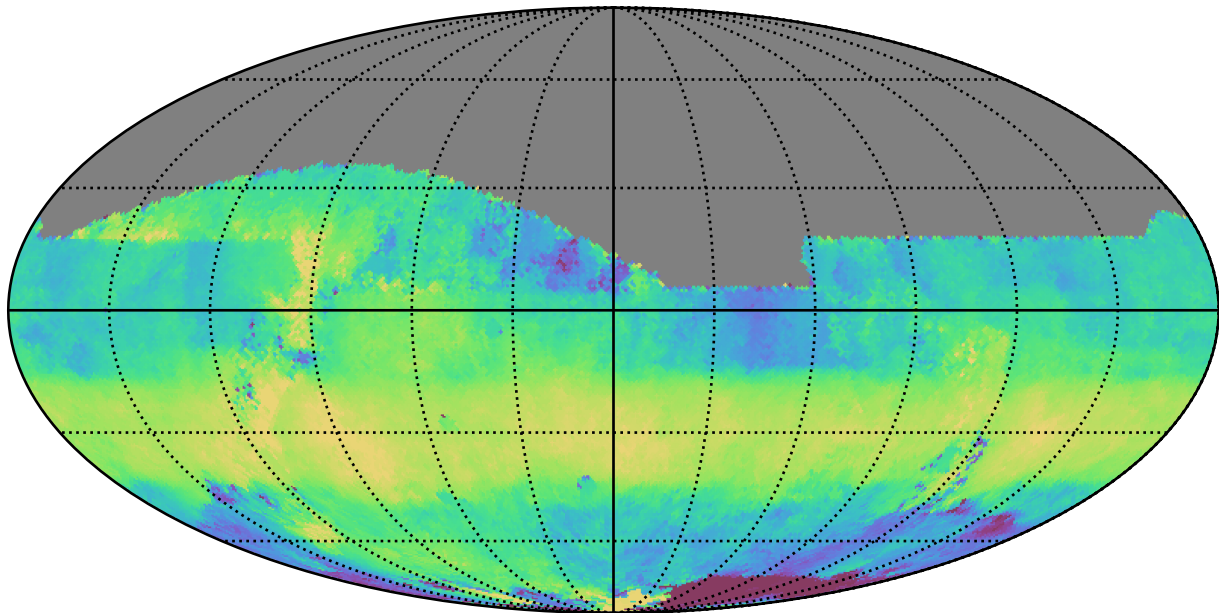
too_elab_r128_d2_griz_v3.4_10yrs All sky z band: Median HA
