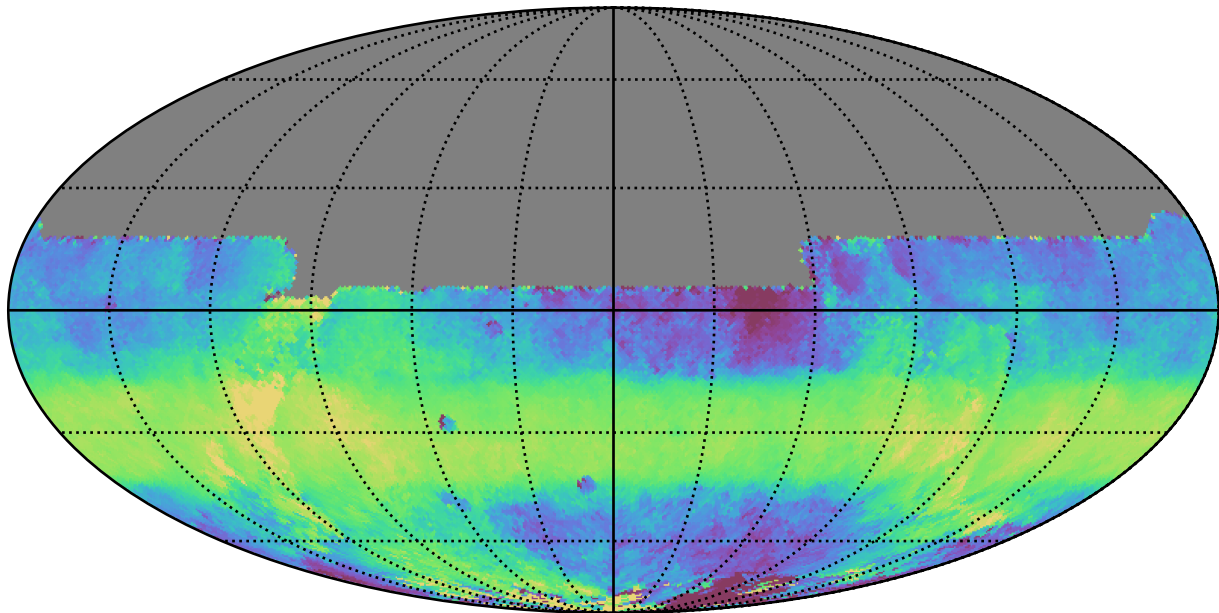
too_elab_r128_d2_griz_v3.4_10yrs All sky y band: Median HA
