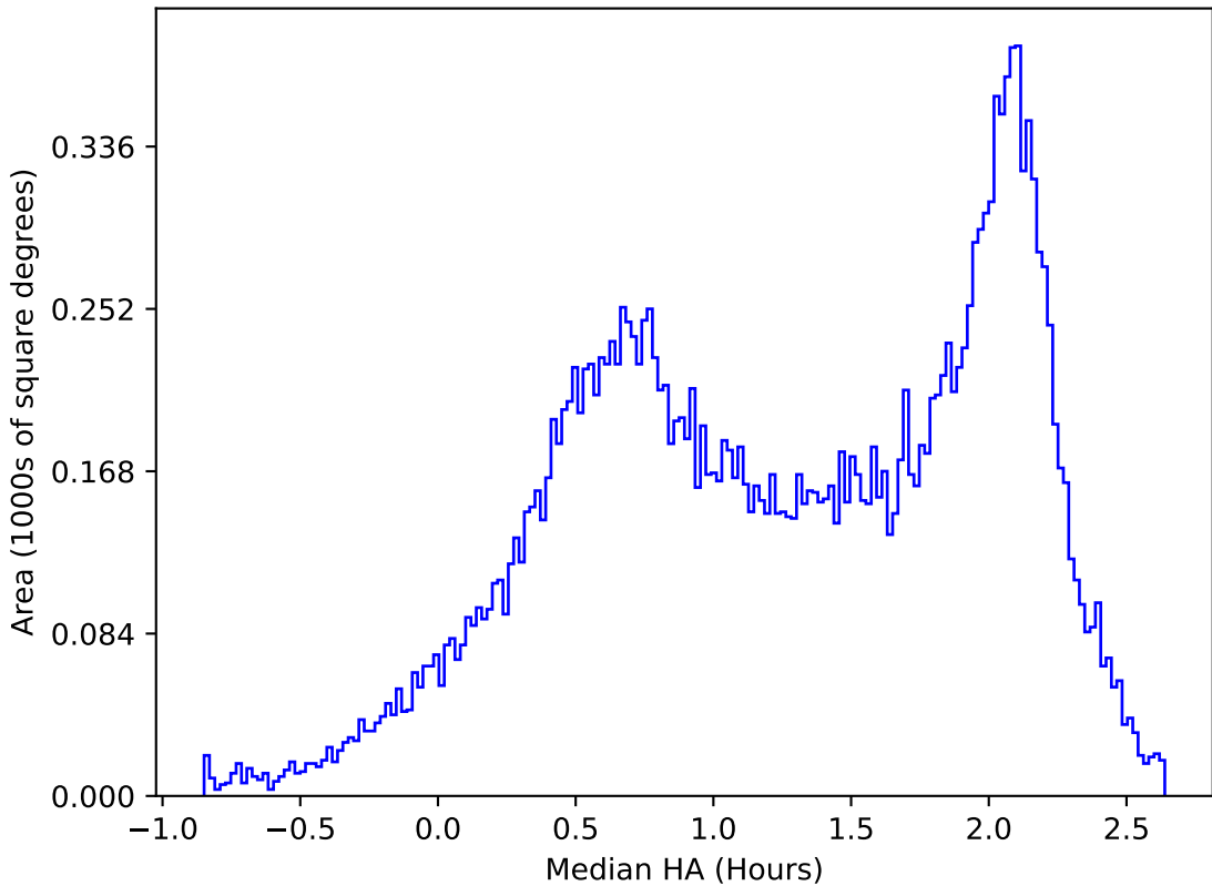
too_elab_r128_d2_griz_v3.4_10yrs All sky y band: Median HA
