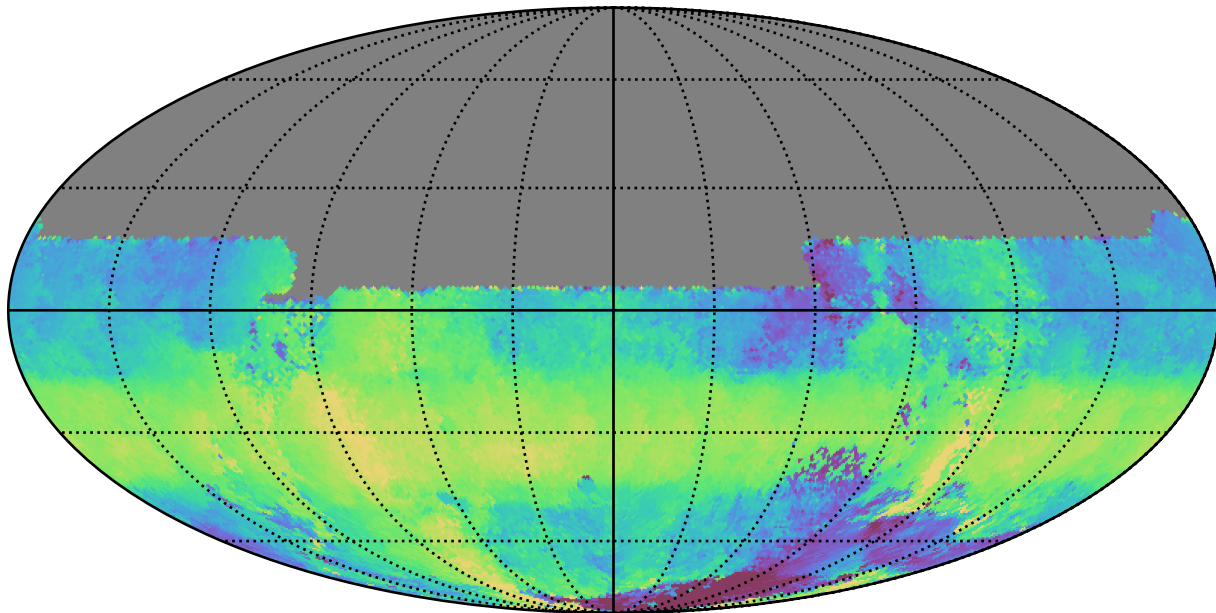
too_elab_r128_d2_griz_v3.4_10yrs All sky u band: Median HA
