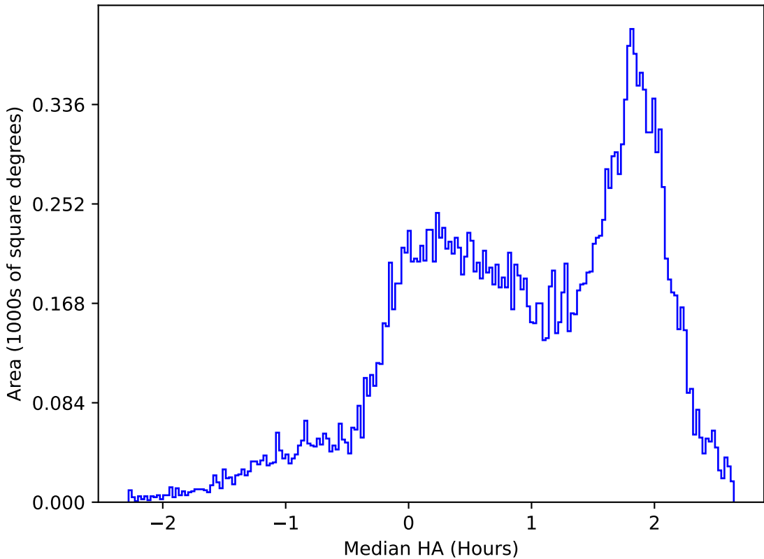
too_elab_r128_d2_griz_v3.4_10yrs All sky u band: Median HA
