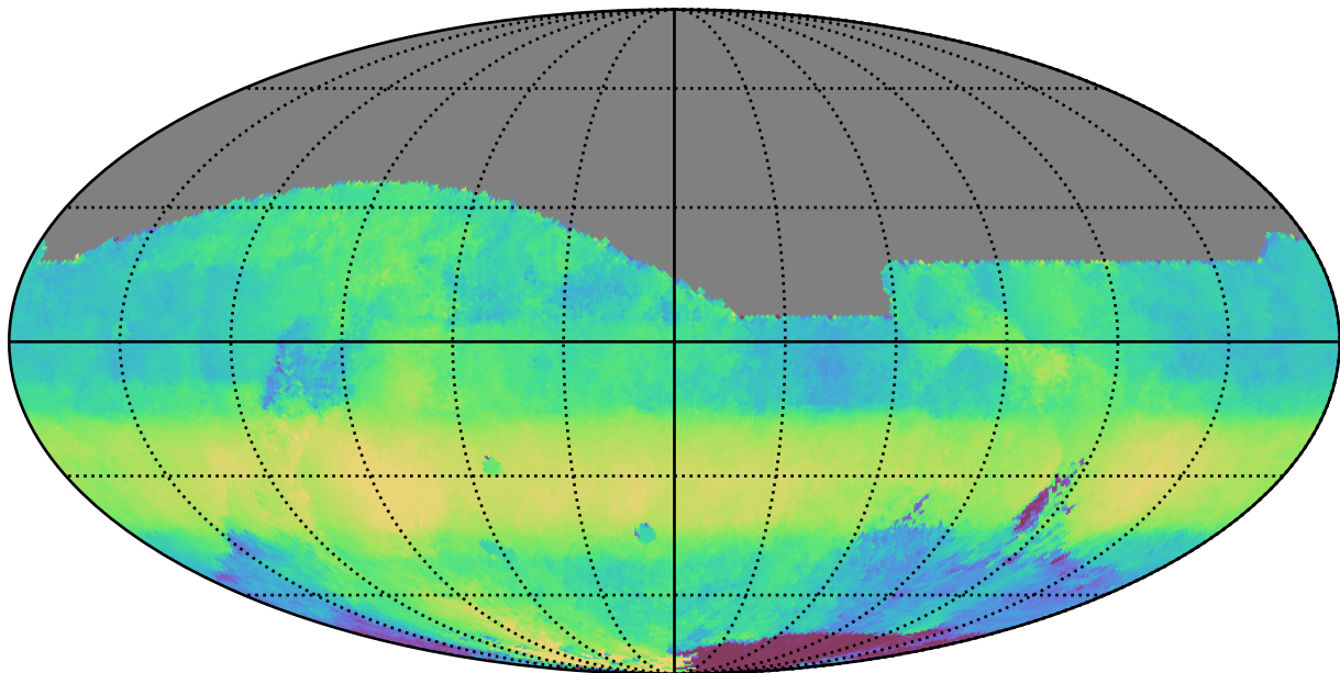
too_elab_r128_d2_griz_v3.4_10yrs All sky r band: Median HA
