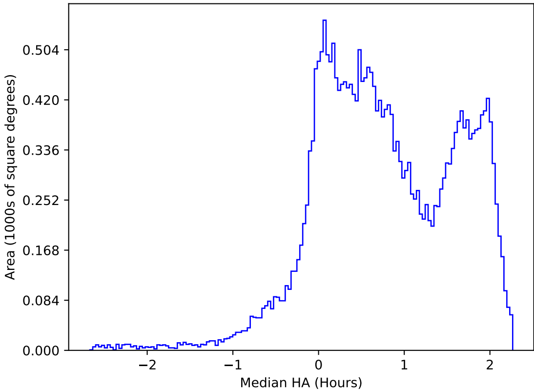
too_elab_r128_d2_griz_v3.4_10yrs All sky r band: Median HA
