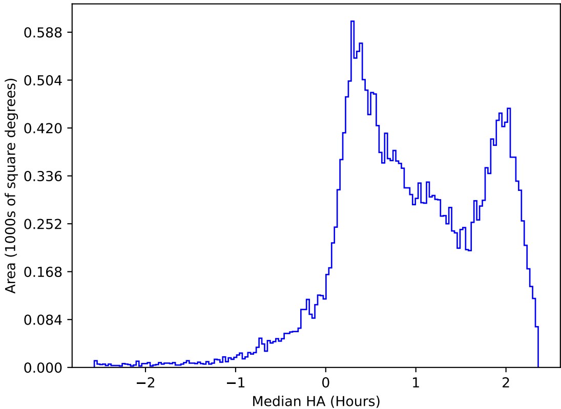
too_elab_r128_d2_griz_v3.4_10yrs All sky i band: Median HA
