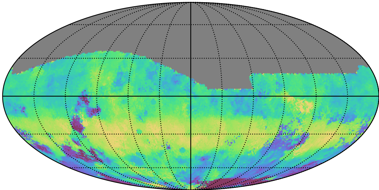
too_elab_r128_d2_griz_v3.4_10yrs All sky g band: Median HA
