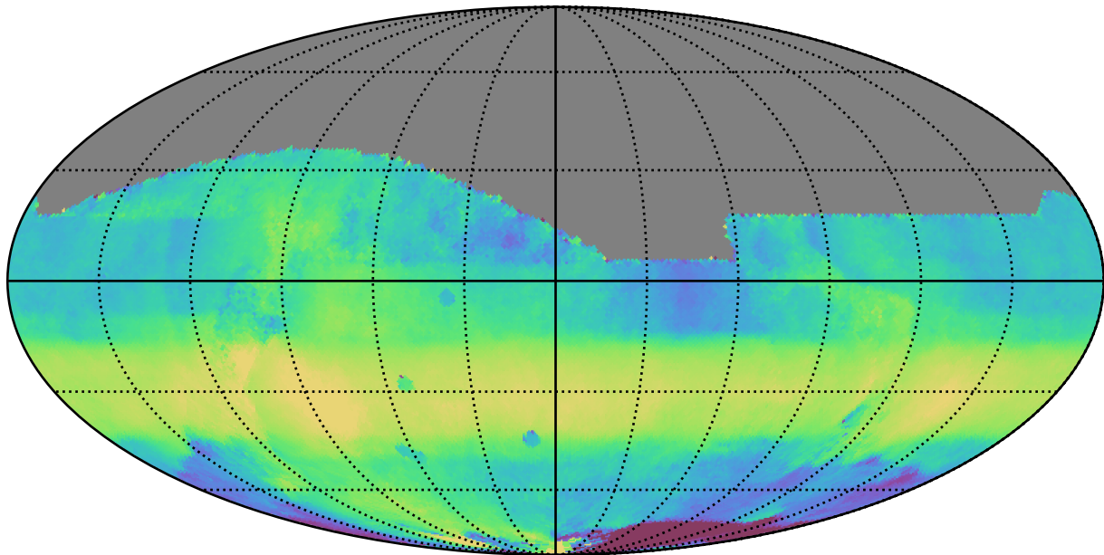
too_elab_r128_d2_griz_v3.4_10yrs All sky all bands: Median HA
