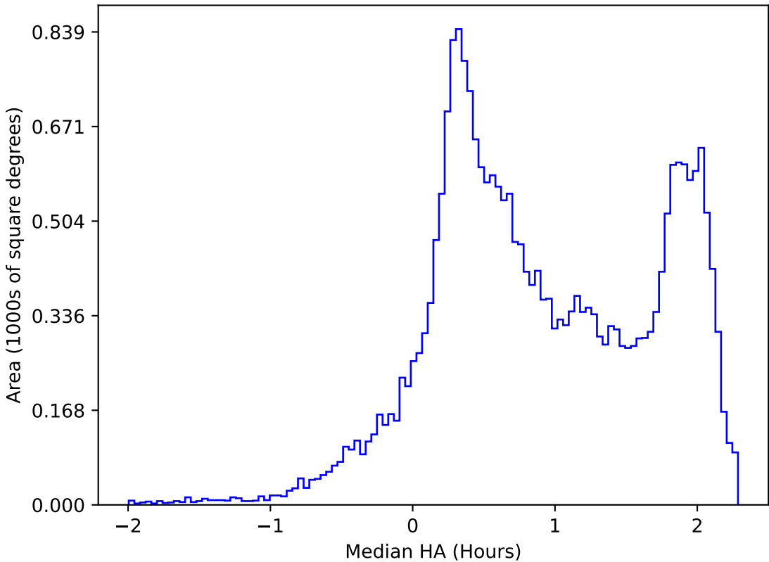
too_elab_r128_d2_griz_v3.4_10yrs All sky all bands: Median HA
