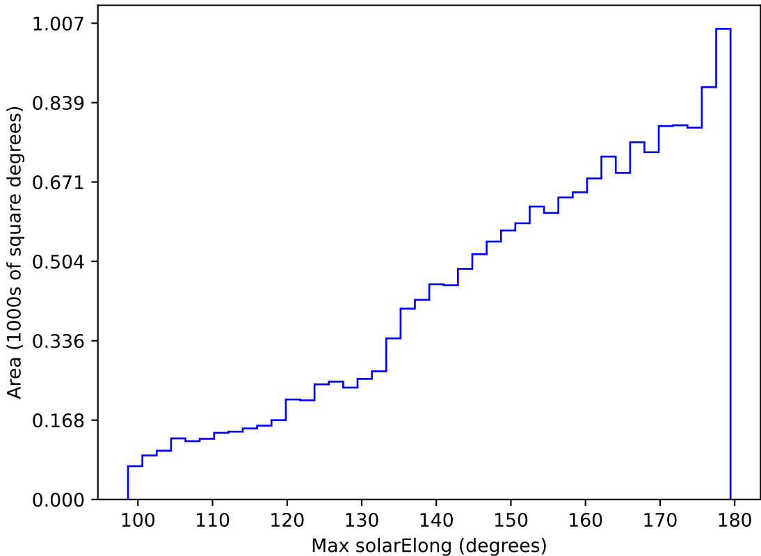
too_elab_r128_d2_griz_v3.4_10yrs WFD z band: Max solarElong
