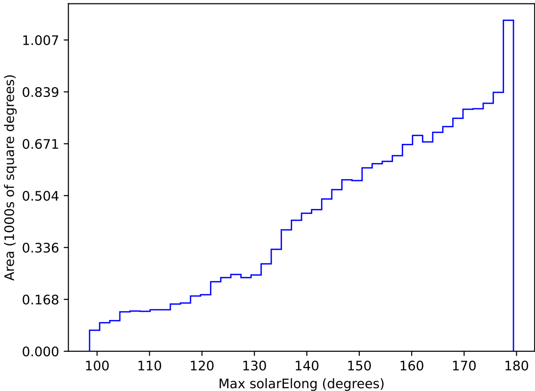
too_elab_r128_d2_griz_v3.4_10yrs WFD r band: Max solarElong
