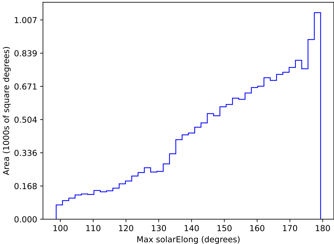
too_elab_r128_d2_griz_v3.4_10yrs WFD i band: Max solarElong
