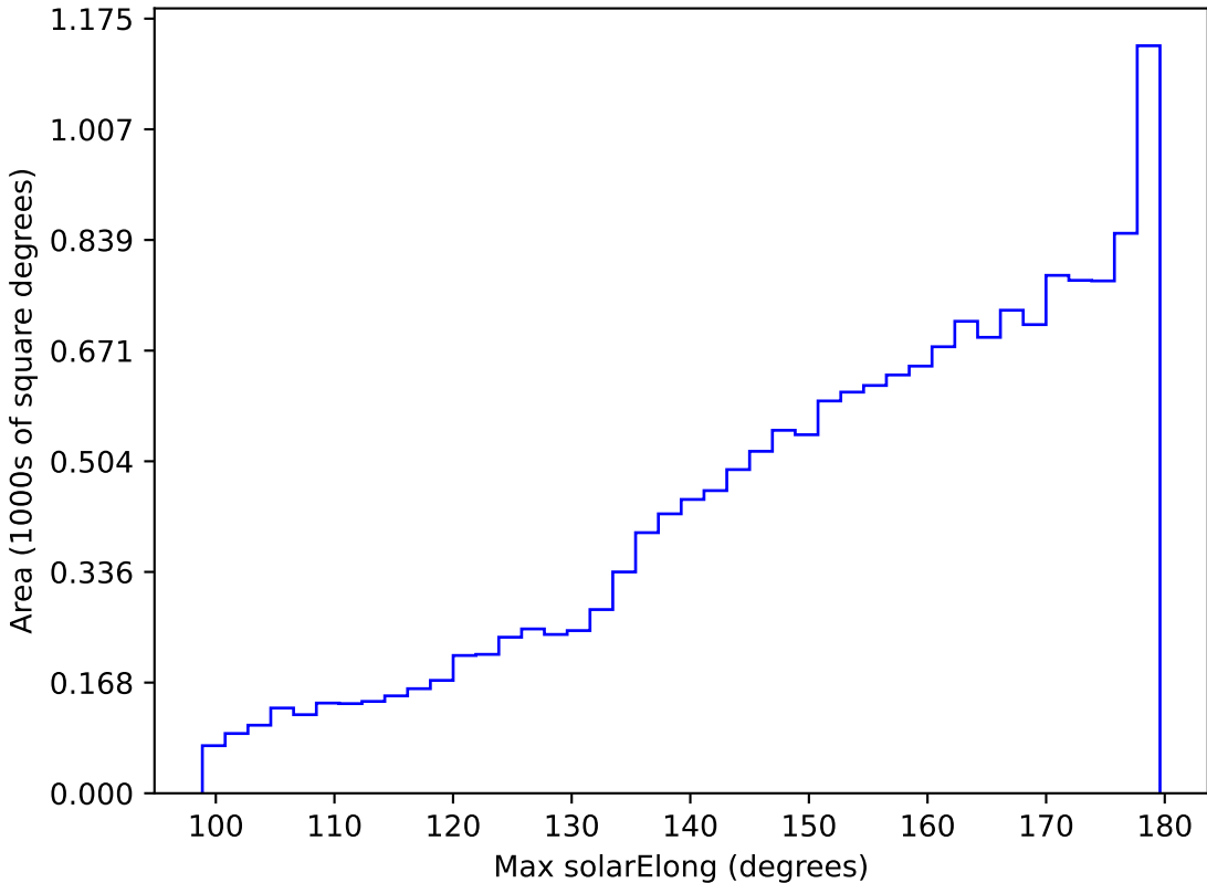
too_elab_r128_d2_griz_v3.4_10yrs WFD all bands: Max solarElong
