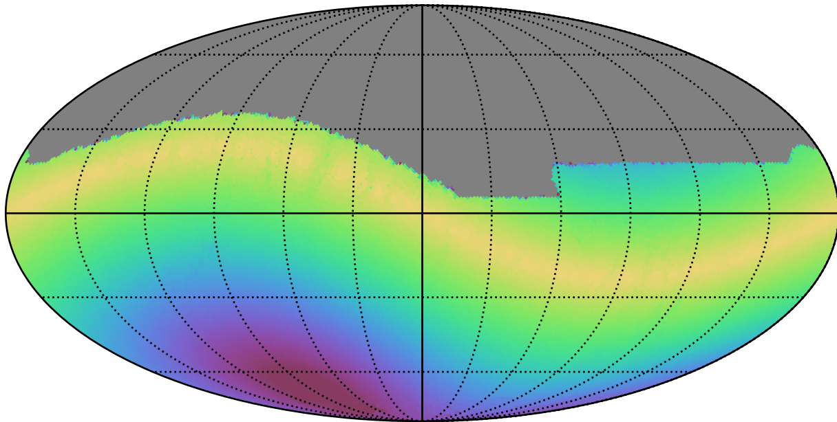
too_elab_r128_d2_griz_v3.4_10yrs All sky z band: Max solarElong
