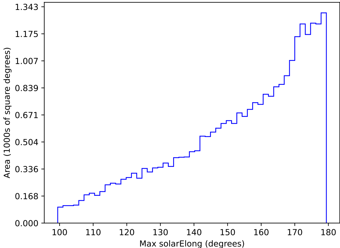
too_elab_r128_d2_griz_v3.4_10yrs All sky z band: Max solarElong
