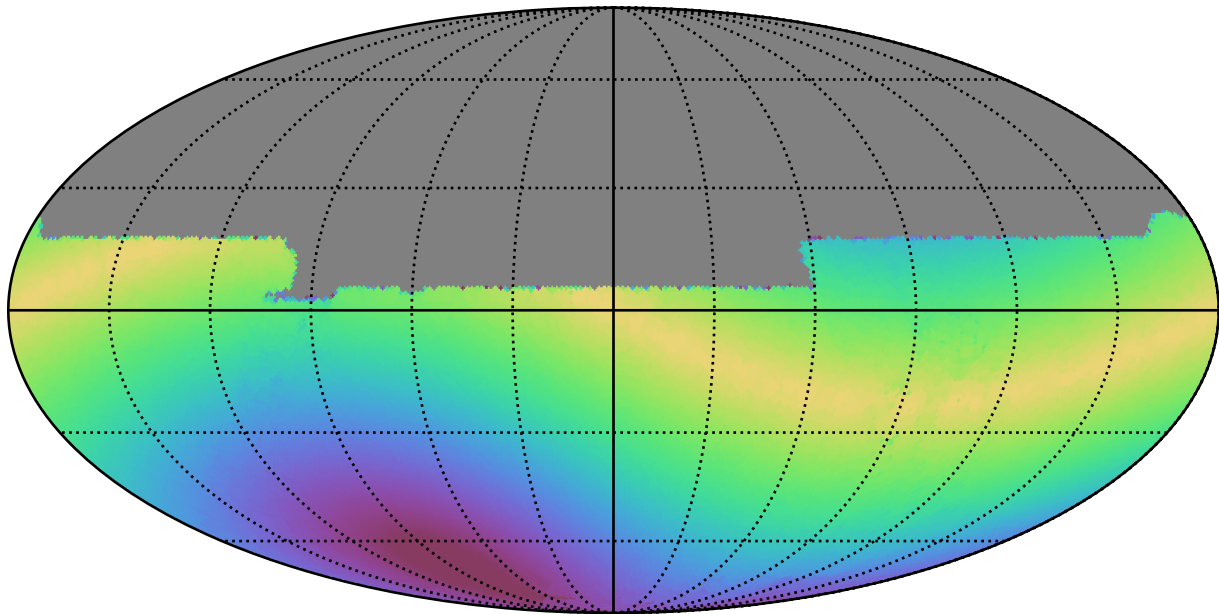
too_elab_r128_d2_griz_v3.4_10yrs All sky y band: Max solarElong
