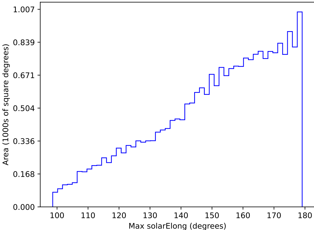
too_elab_r128_d2_griz_v3.4_10yrs All sky y band: Max solarElong
