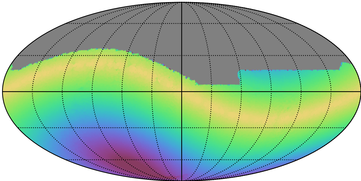
too_elab_r128_d2_griz_v3.4_10yrs All sky r band: Max solarElong
