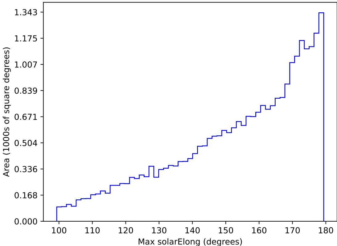
too_elab_r128_d2_griz_v3.4_10yrs All sky r band: Max solarElong
