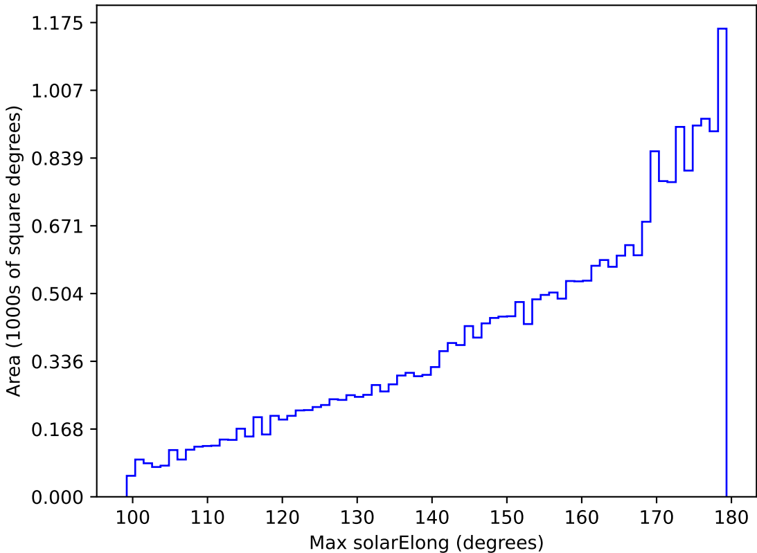
too_elab_r128_d2_griz_v3.4_10yrs All sky i band: Max solarElong
