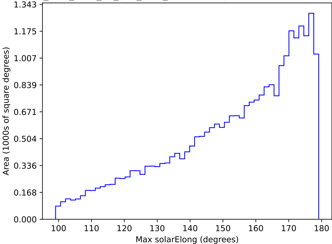
too_elab_r128_d2_griz_v3.4_10yrs All sky g band: Max solarElong
