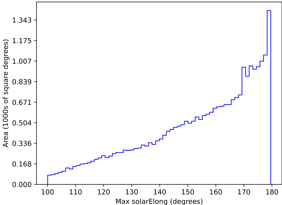
too_elab_r128_d2_griz_v3.4_10yrs All sky all bands: Max solarElong
