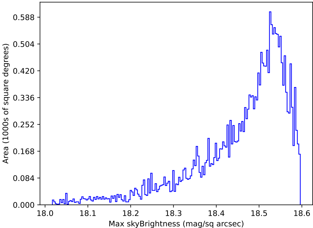
too_elab_r128_d2_griz_v3.4_10yrs Yr 1 y band: Max skyBrightness
