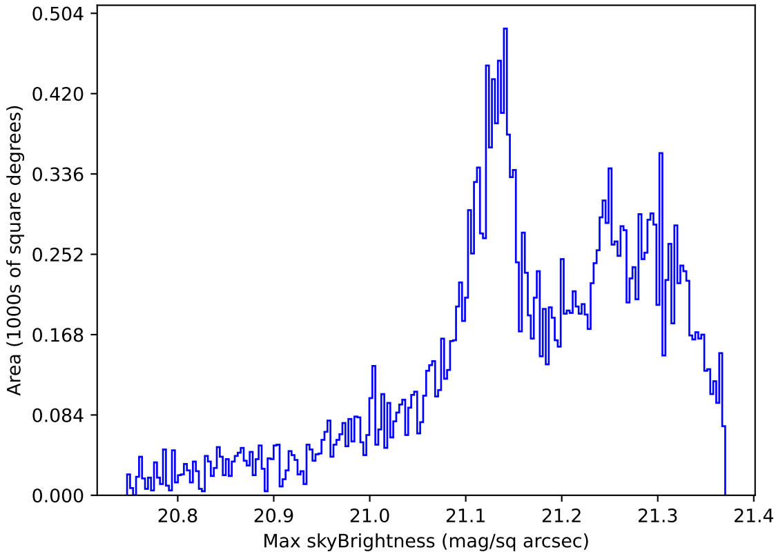
too_elab_r128_d2_griz_v3.4_10yrs Yr 1 r band: Max skyBrightness
