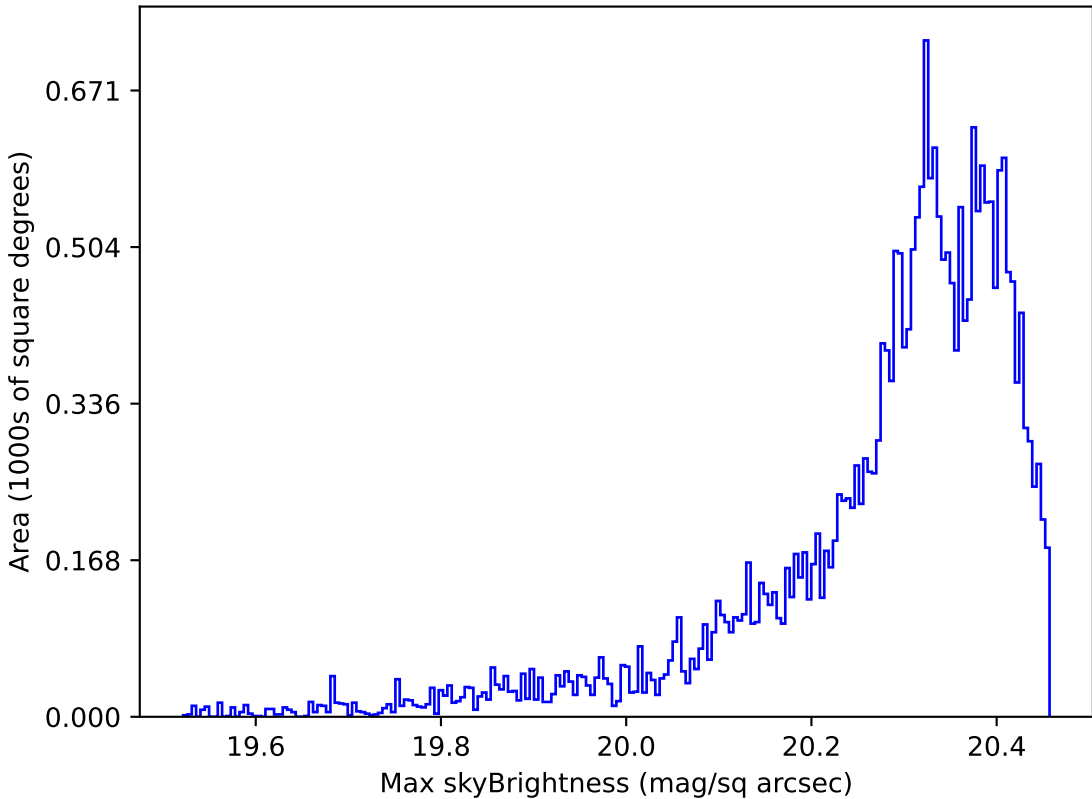
too_elab_r128_d2_griz_v3.4_10yrs Yr 1 i band: Max skyBrightness
