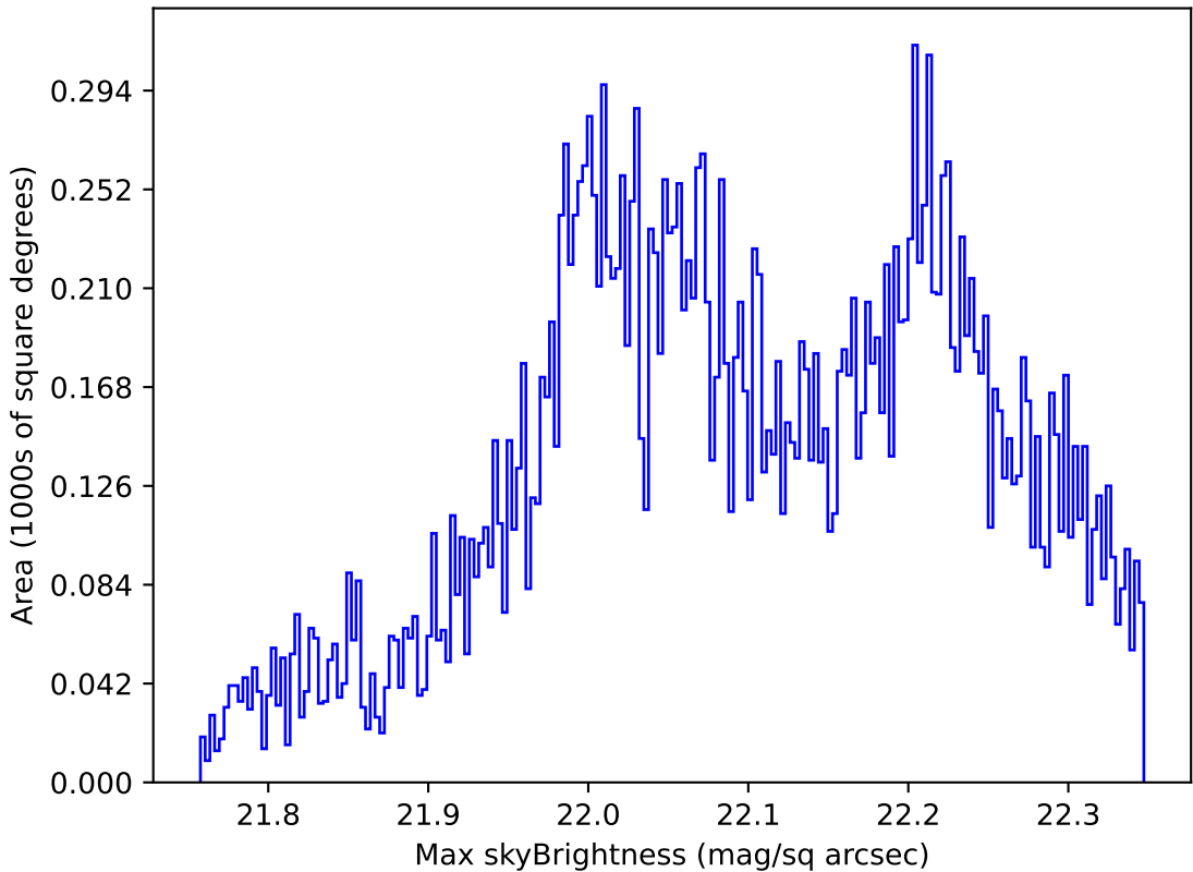
too_elab_r128_d2_griz_v3.4_10yrs Yr 1 g band: Max skyBrightness
