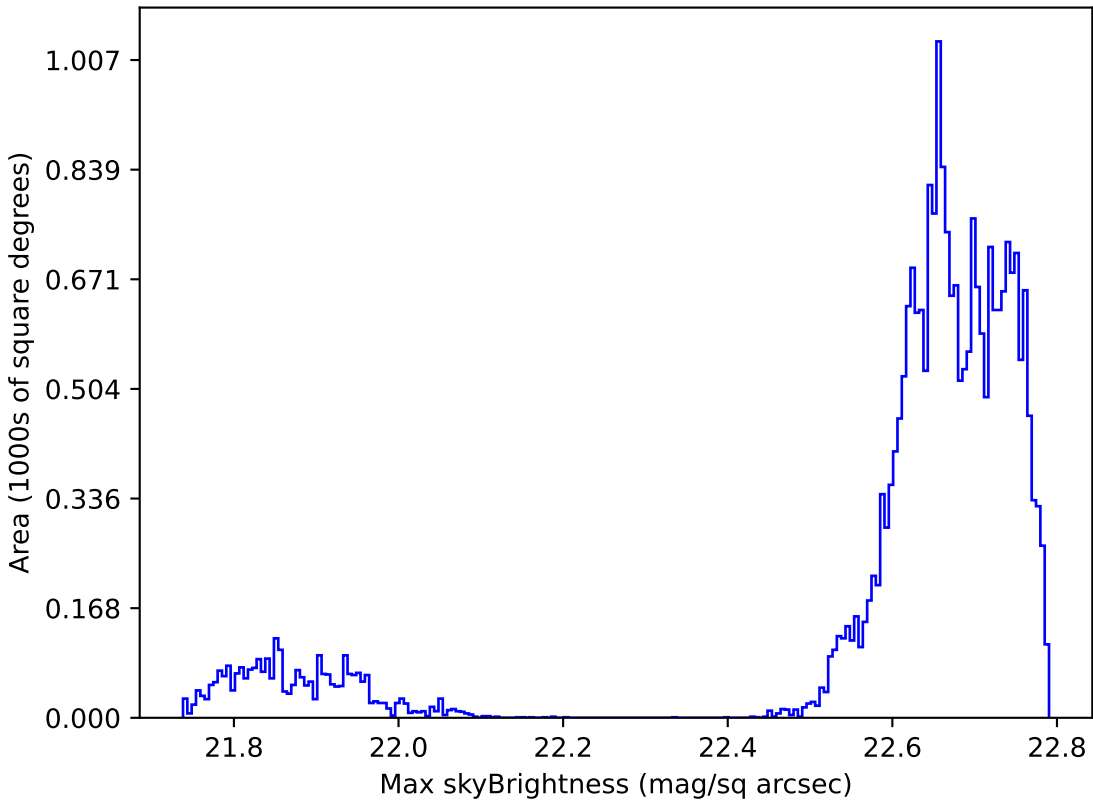
too_elab_r128_d2_griz_v3.4_10yrs Yr 1 all bands: Max skyBrightness
