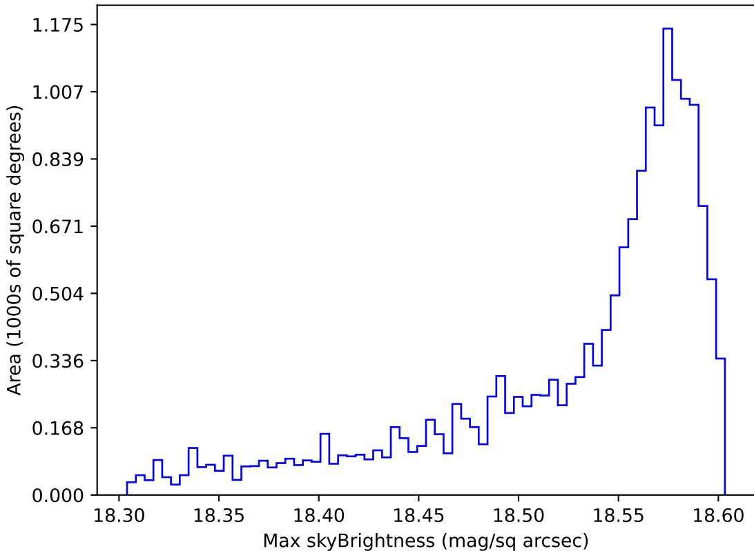
too_elab_r128_d2_griz_v3.4_10yrs WFD y band: Max skyBrightness
