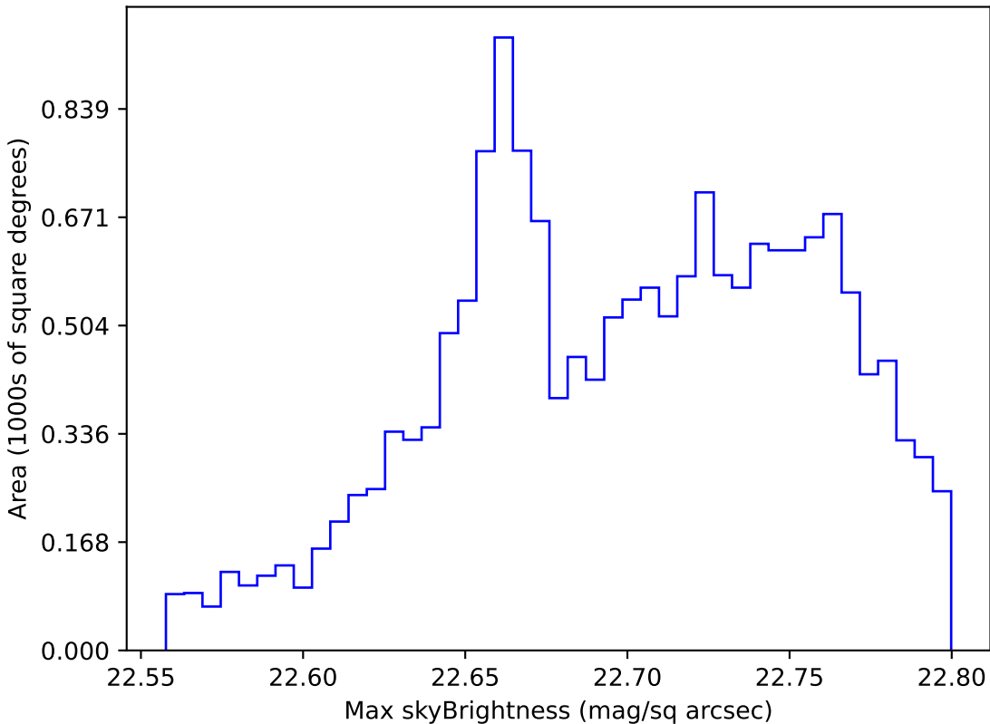
too_elab_r128_d2_griz_v3.4_10yrs WFD u band: Max skyBrightness
