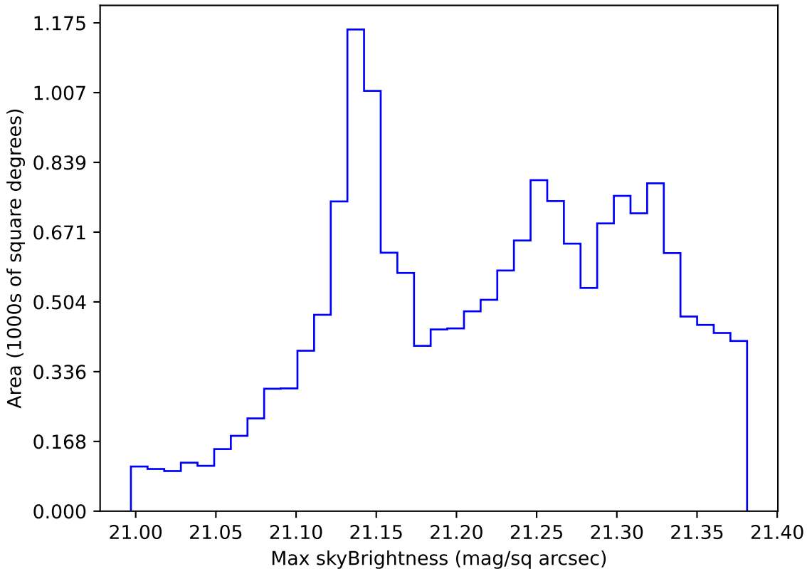
too_elab_r128_d2_griz_v3.4_10yrs WFD r band: Max skyBrightness
