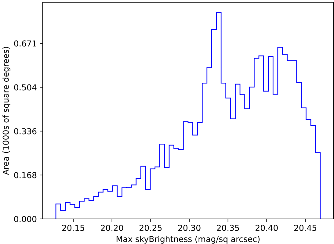
too_elab_r128_d2_griz_v3.4_10yrs WFD i band: Max skyBrightness
