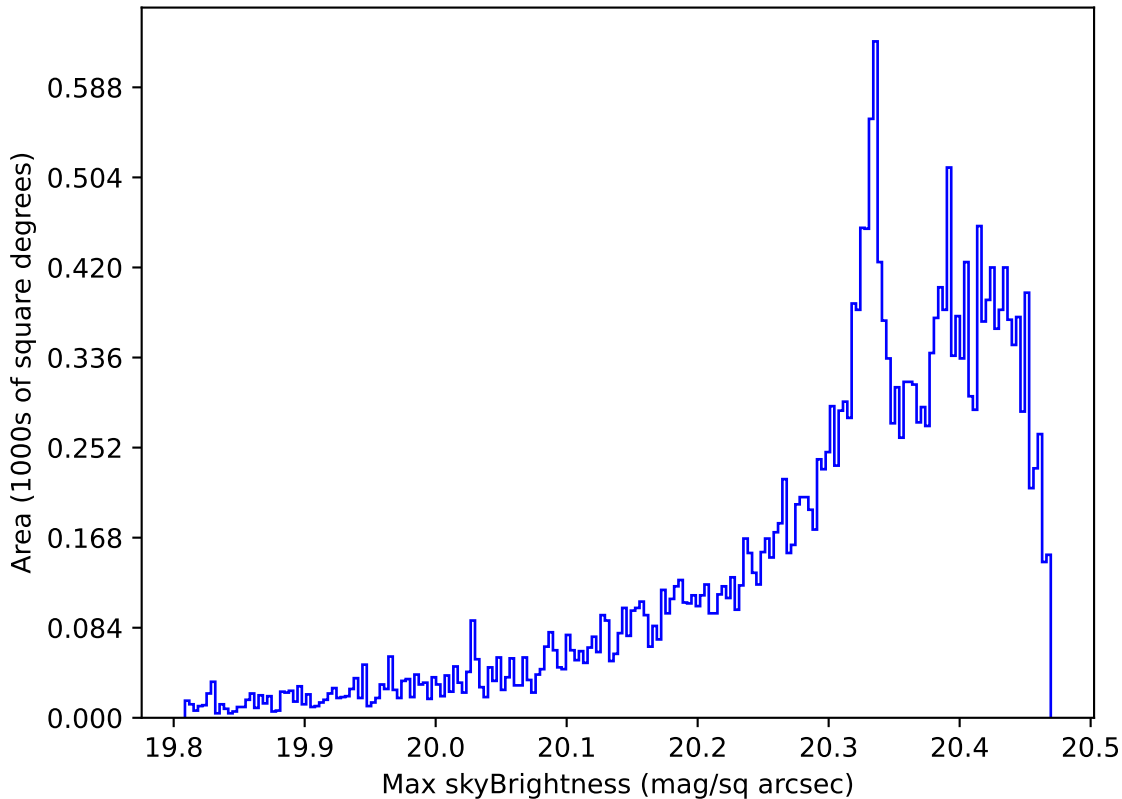
too_elab_r128_d2_griz_v3.4_10yrs All sky i band: Max skyBrightness
