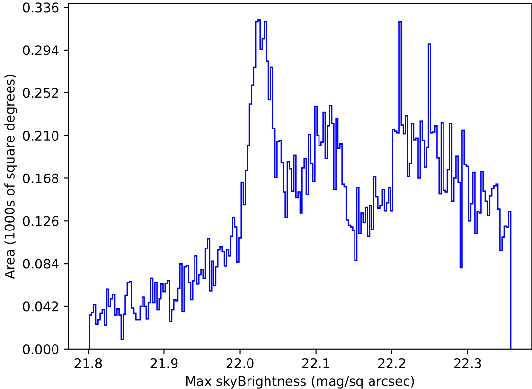
too_elab_r128_d2_griz_v3.4_10yrs All sky g band: Max skyBrightness
