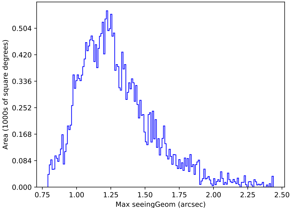
too_elab_r128_d2_griz_v3.4_10yrs Yr 1 z band: Max seeingGeom
