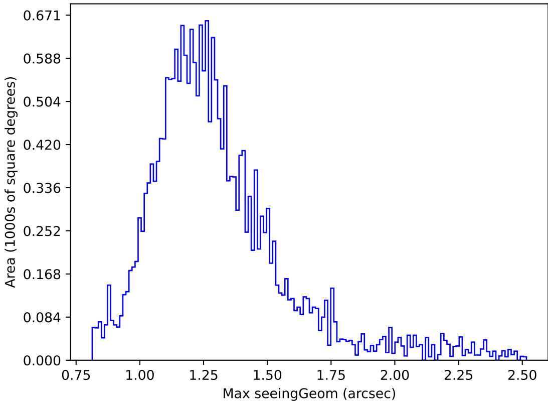
too_elab_r128_d2_griz_v3.4_10yrs Yr 1 y band: Max seeingGeom
