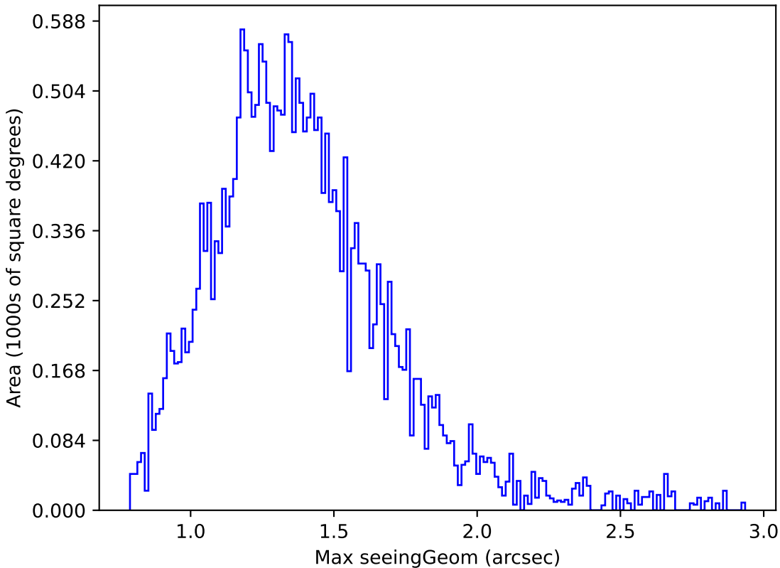
too_elab_r128_d2_griz_v3.4_10yrs Yr 1 r band: Max seeingGeom
