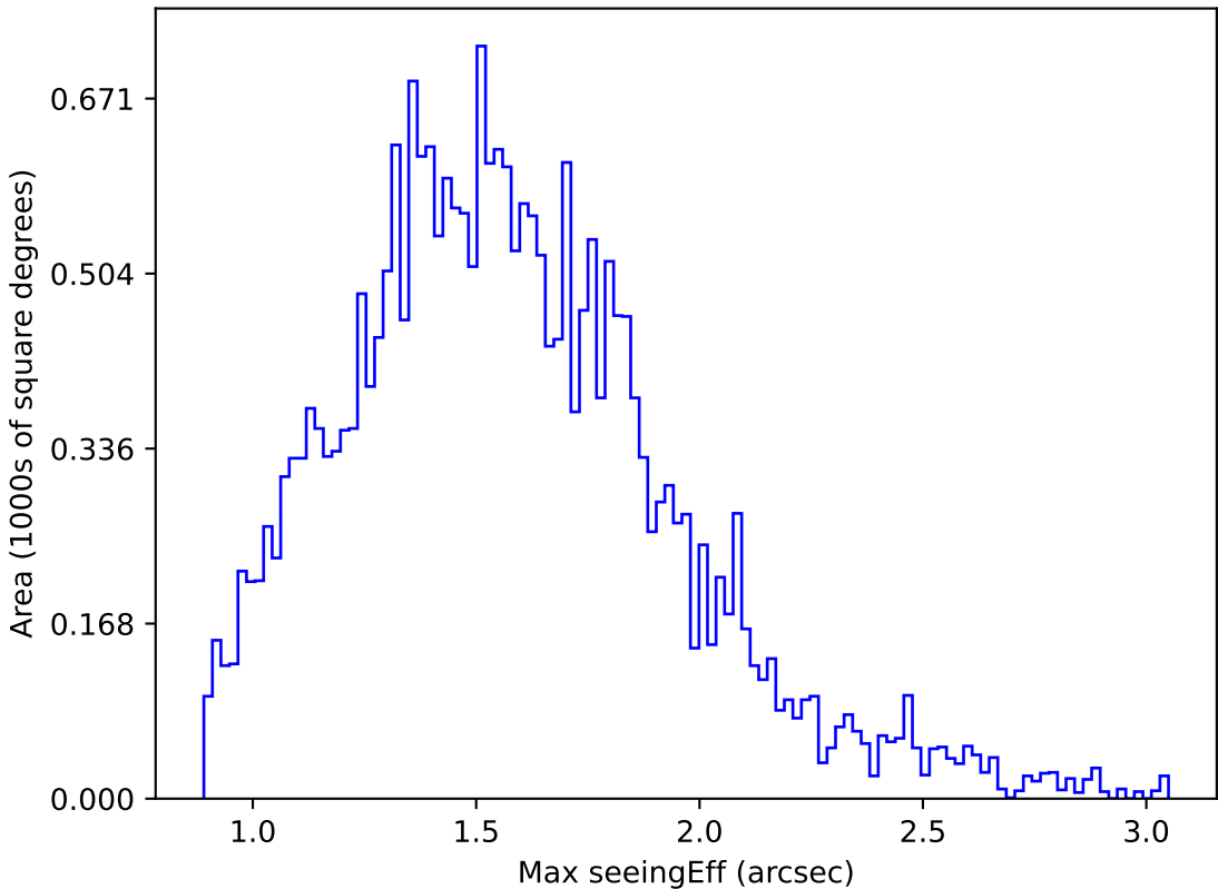
too_elab_r128_d2_griz_v3.4_10yrs Yr 1 g band: Max seeingEff
