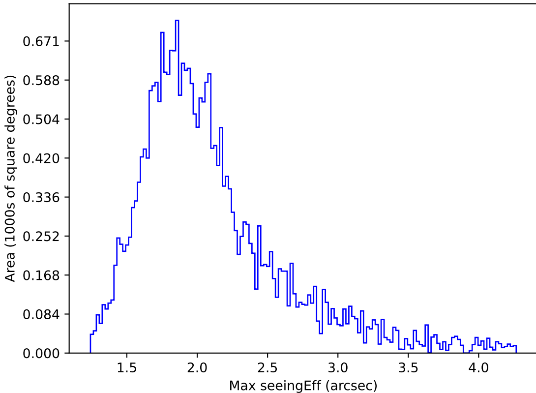
too_elab_r128_d2_griz_v3.4_10yrs Yr 1 all bands: Max seeingEff
