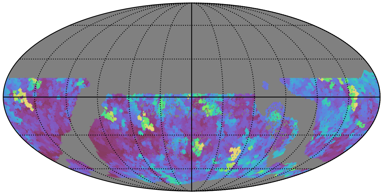
too_elab_r128_d2_griz_v3.4_10yrs WFD z band: Max seeingEff
