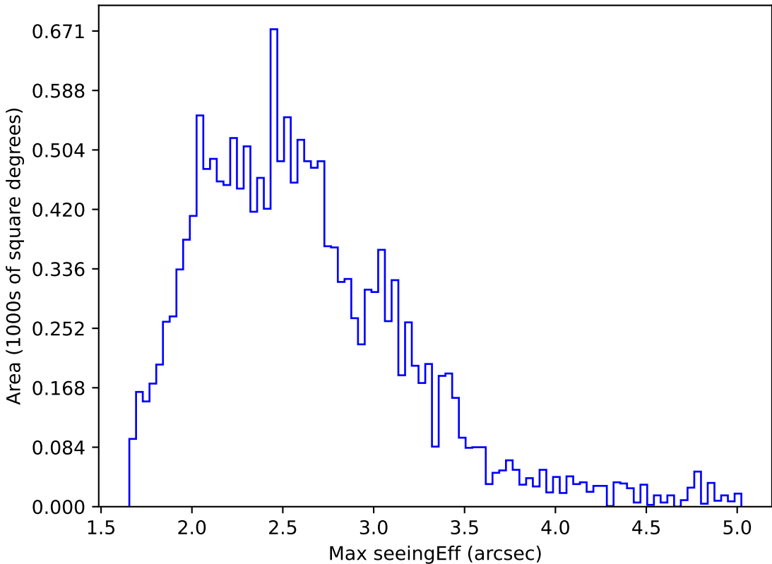
too_elab_r128_d2_griz_v3.4_10yrs WFD z band: Max seeingEff
