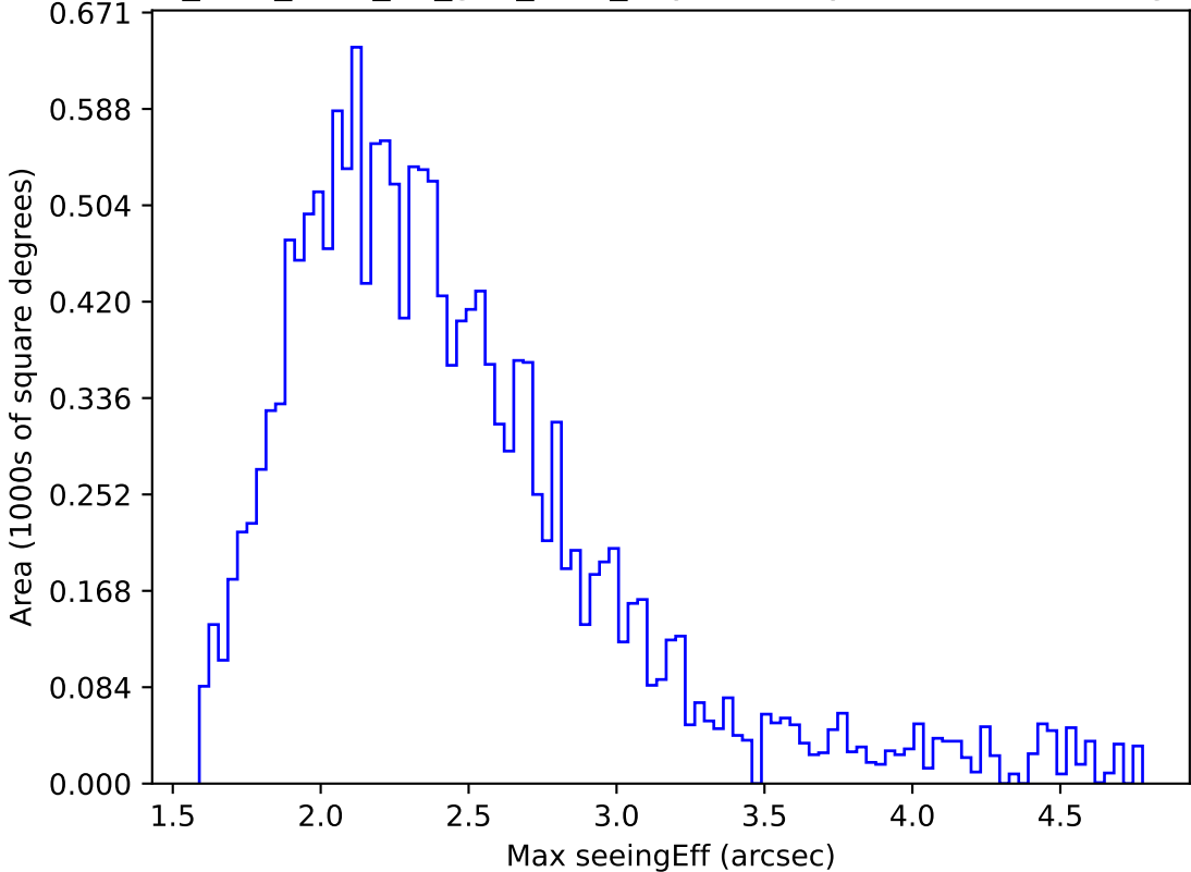
too_elab_r128_d2_griz_v3.4_10yrs WFD y band: Max seeingEff
