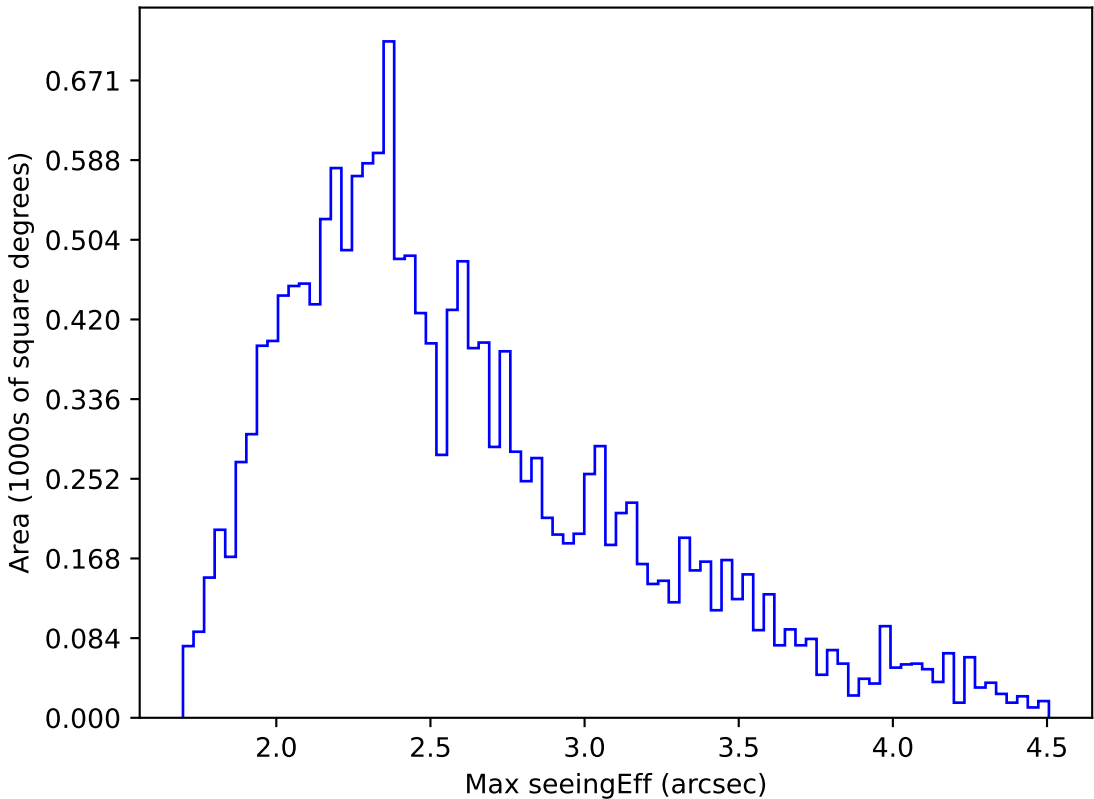
too_elab_r128_d2_griz_v3.4_10yrs WFD u band: Max seeingEff
