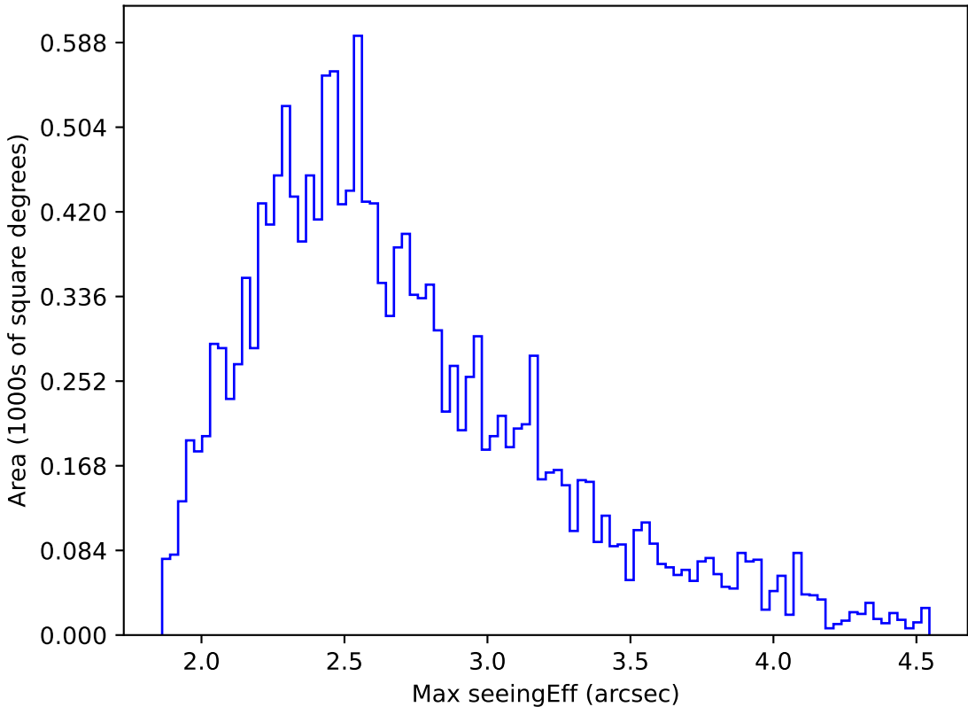
too_elab_r128_d2_griz_v3.4_10yrs WFD r band: Max seeingEff
