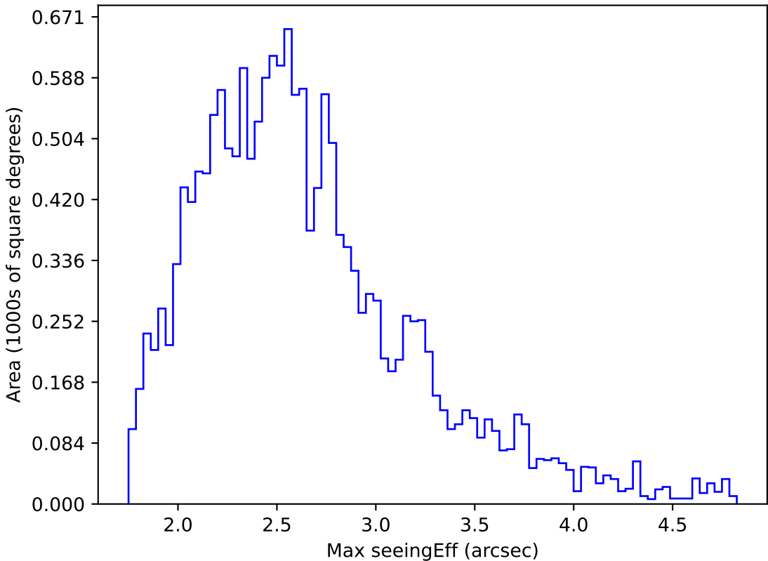
too_elab_r128_d2_griz_v3.4_10yrs WFD i band: Max seeingEff
