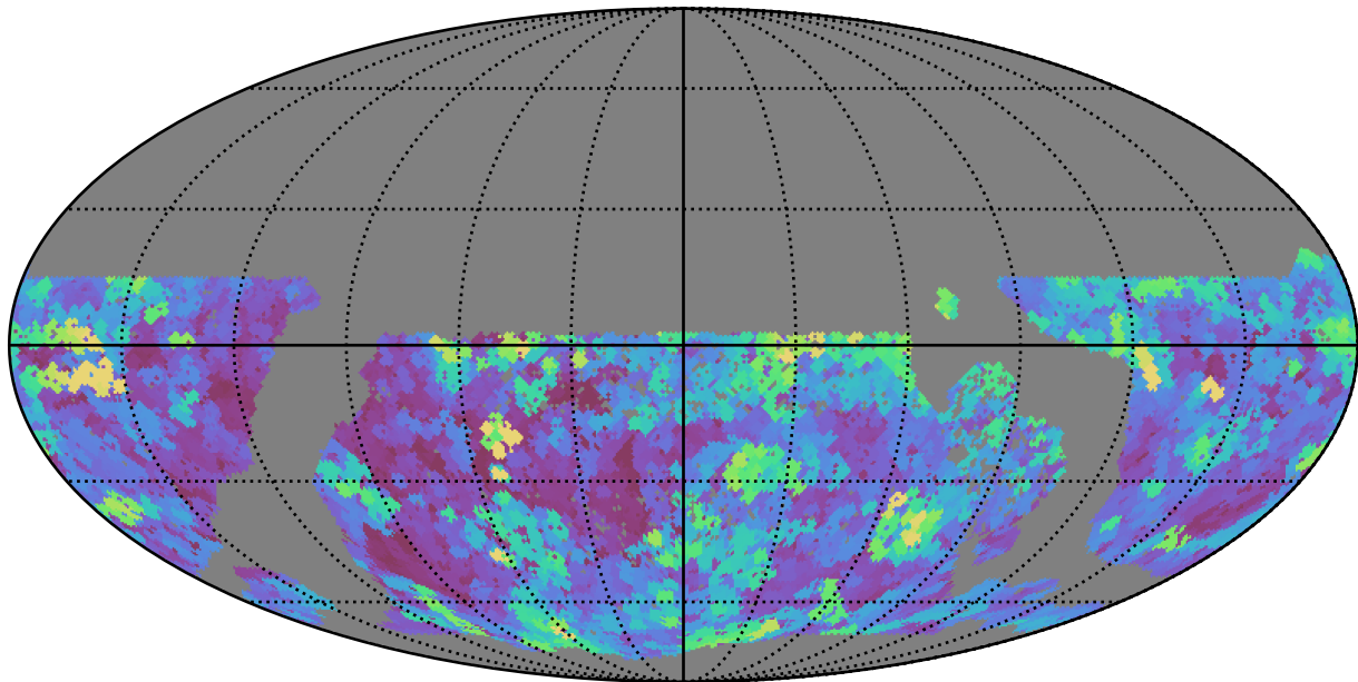
too_elab_r128_d2_griz_v3.4_10yrs WFD g band: Max seeingEff
