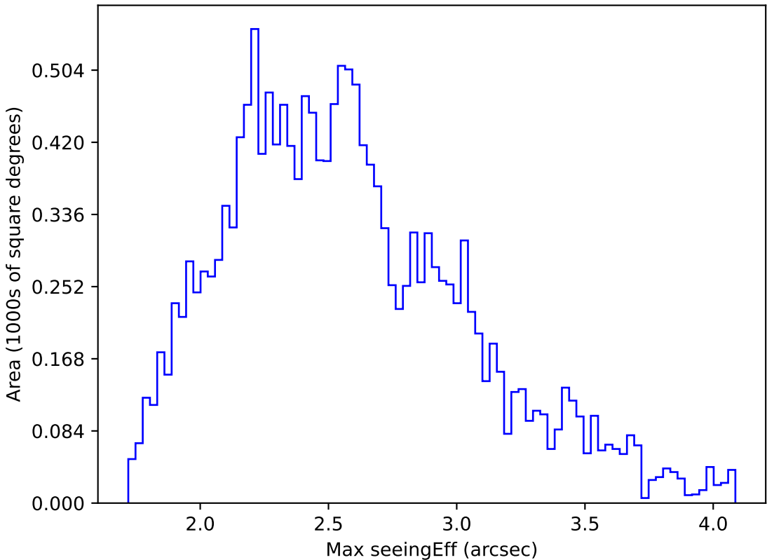
too_elab_r128_d2_griz_v3.4_10yrs WFD g band: Max seeingEff
